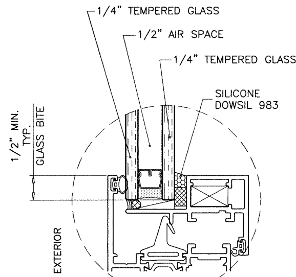
GLAZING DETAIL 1" OVERALL INSUL. GLASS
