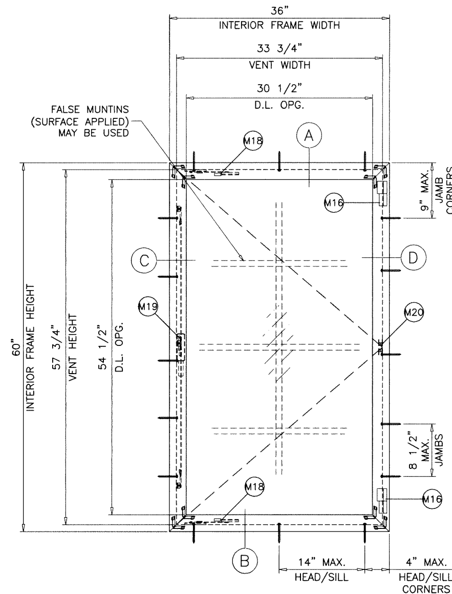
TYPICAL ELEVATION ANCHORS THRU WDW. FRAMES
