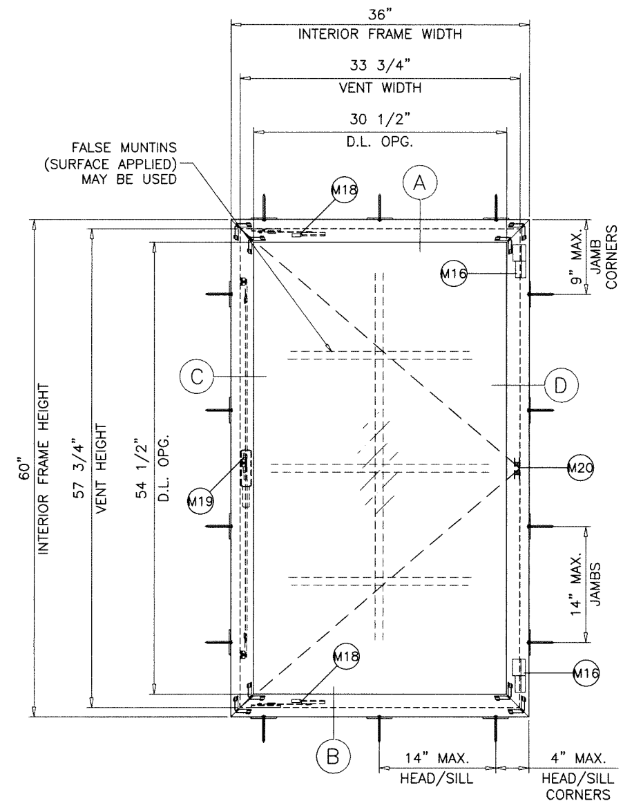
TYPICAL ELEVATION ANCHORS THRU STRAP CLIPS
